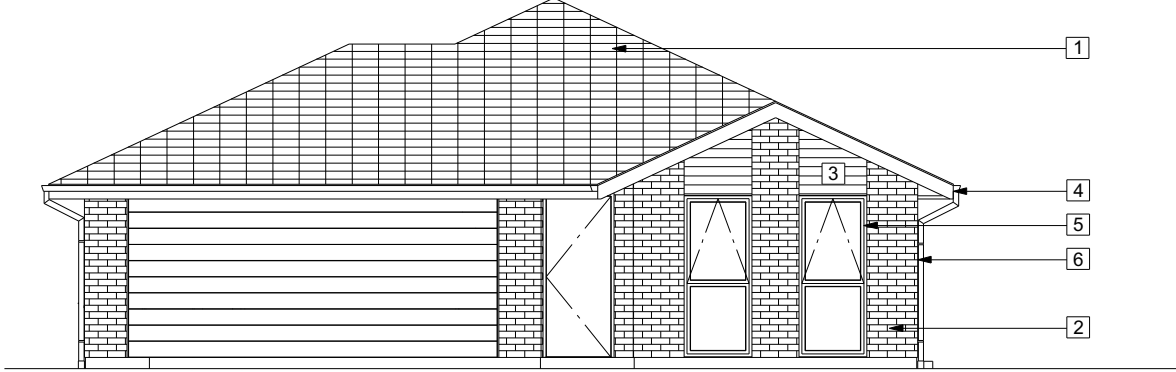
A 4 ELEVATION A 1:100
