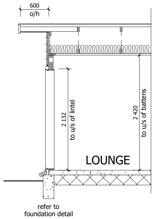
C SECTION 4 1.50
