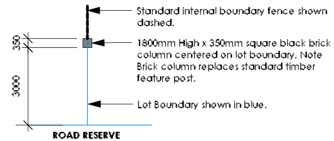
ROAD 3 - TYPICAL BRICK COLUMN DETAIL (Lots 175 - 185 & 199 - 209)
